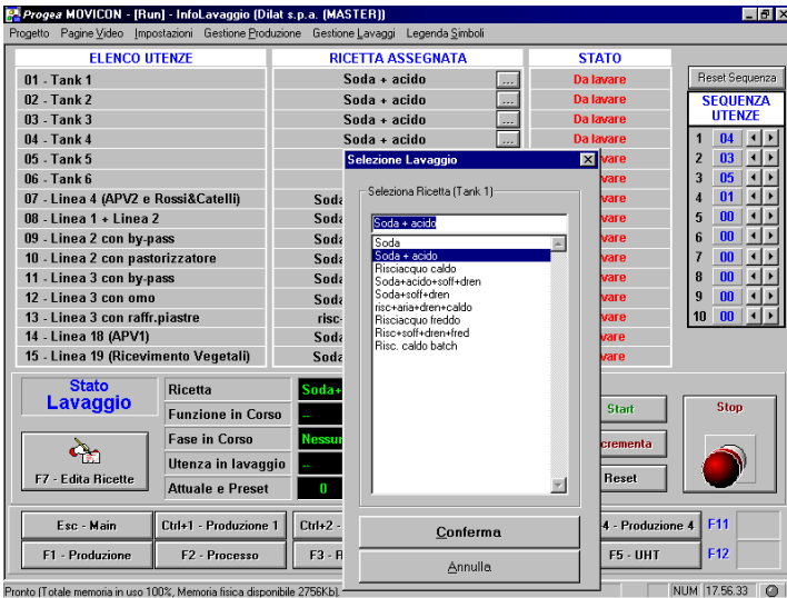
fig. 5: The operator can set consecutive washes by associating each different piece of plant equipment with a different cleaning recipe.
